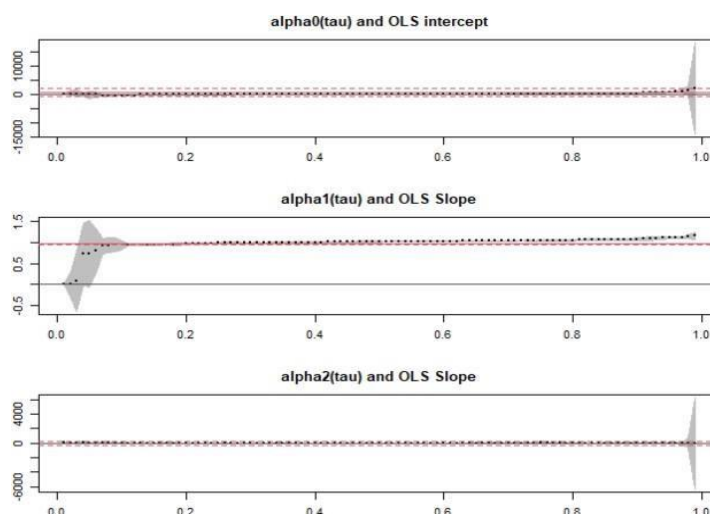
Figure 4. Quantile Autoregression (QAR) Coefficients and Ordinary Least Squares (OLS) Estimates for the Effect of FDI Inflow on Carbon (CO 2 ) Emissions
